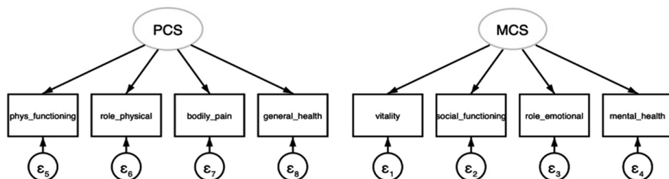
Figure 1 THE STRUCTURAL EQUATION MODEL FOR THE FACTOR ANALYSIS
